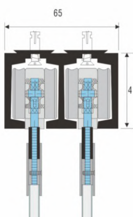
OS-AT-2 Double Sliding Track in 12 Feet
