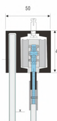
OS-AT-3 Fix + Sliding Track in 12 Feet
