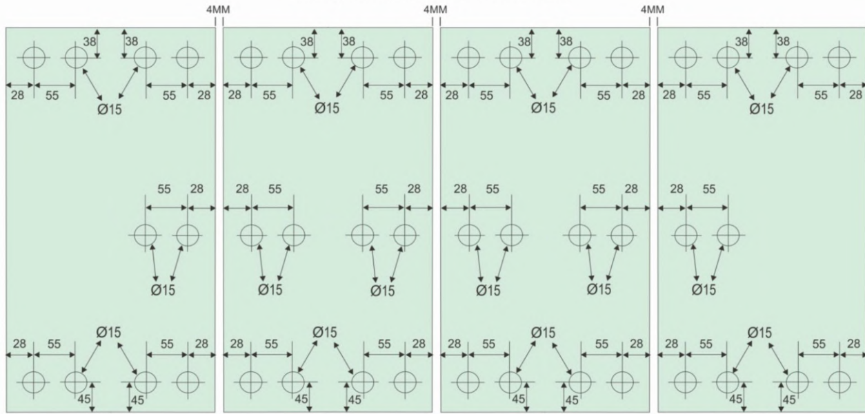
Sliding Folding System B 4 Glass Panel
