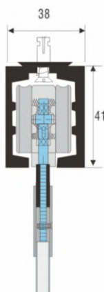
OS-AT-1 Single Sliding Track in 12 Feet
