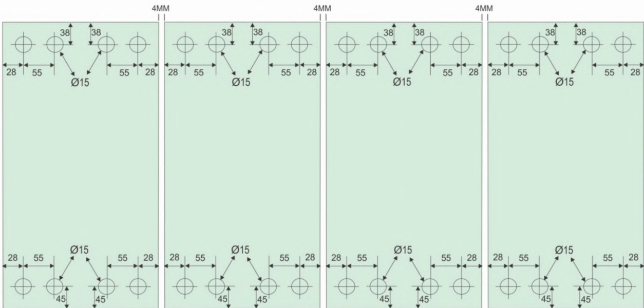
Sliding Folding System A 4 Glass Panel
