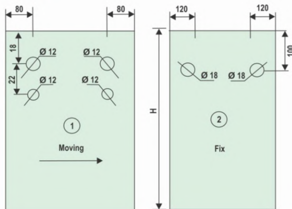
10x30 mm Track
